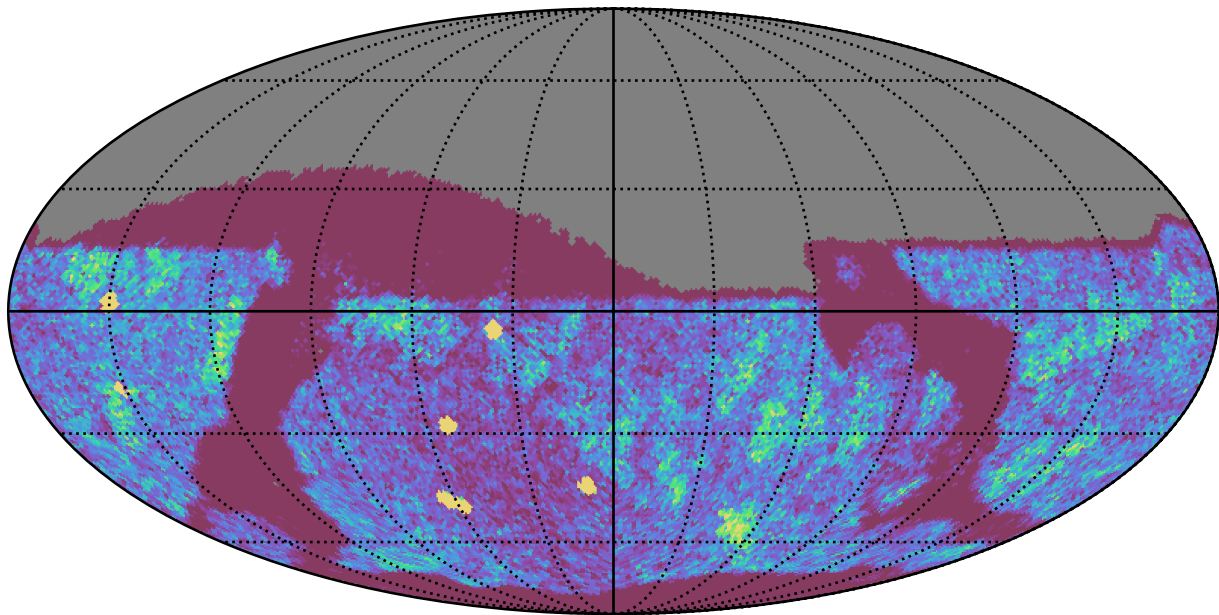
ddf_loaded_fl15_v3.4_10yrs Yr 1 z band: NVisits
