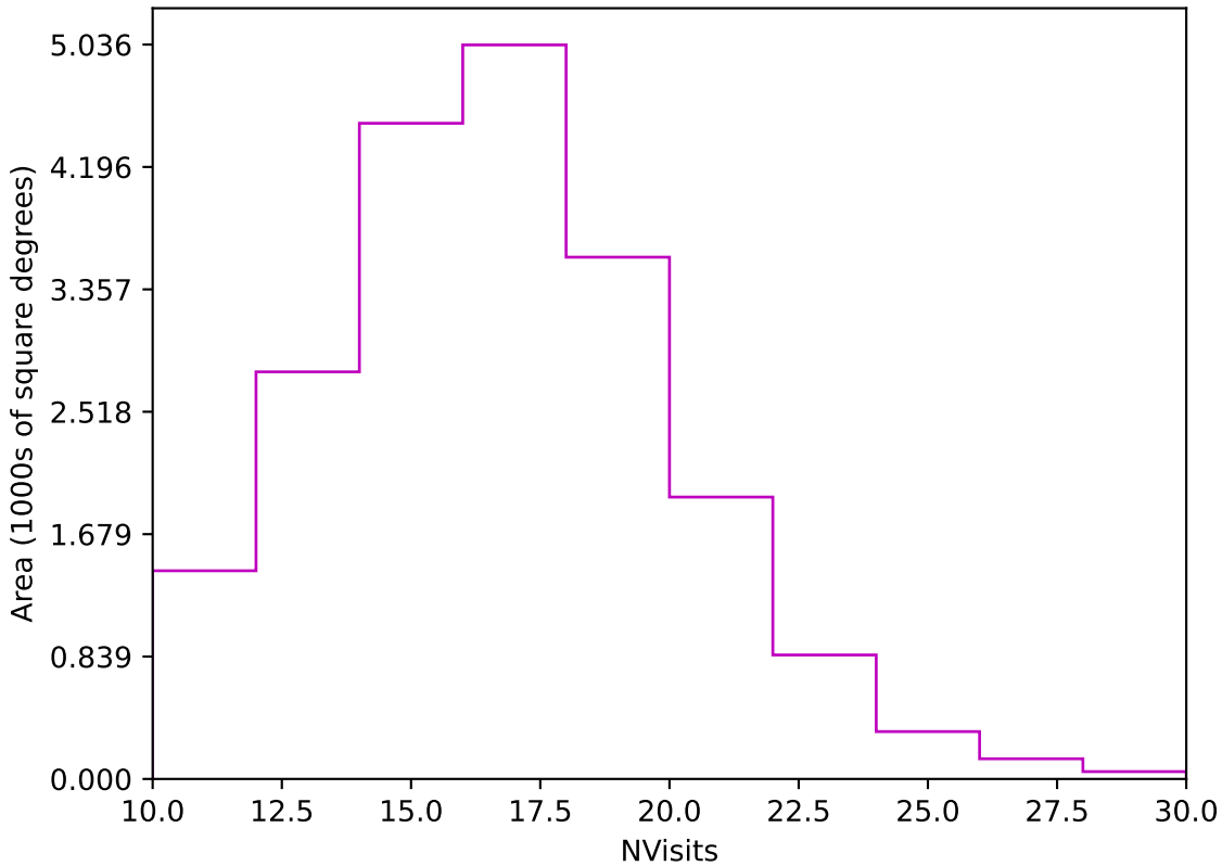
ddf_loaded_fl15_v3.4_10yrs Yr 1 z band: NVisits
