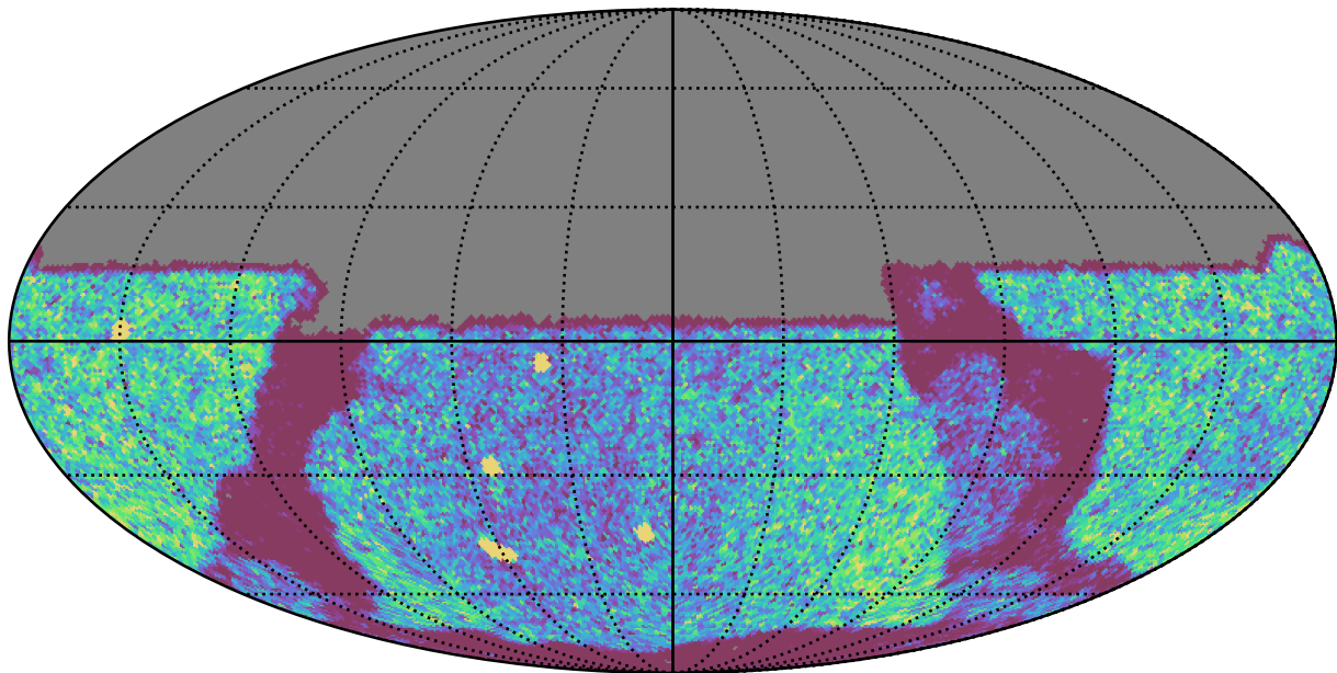
ddf_loaded_fl15_v3.4_10yrs Yr 1 y band: NVisits
