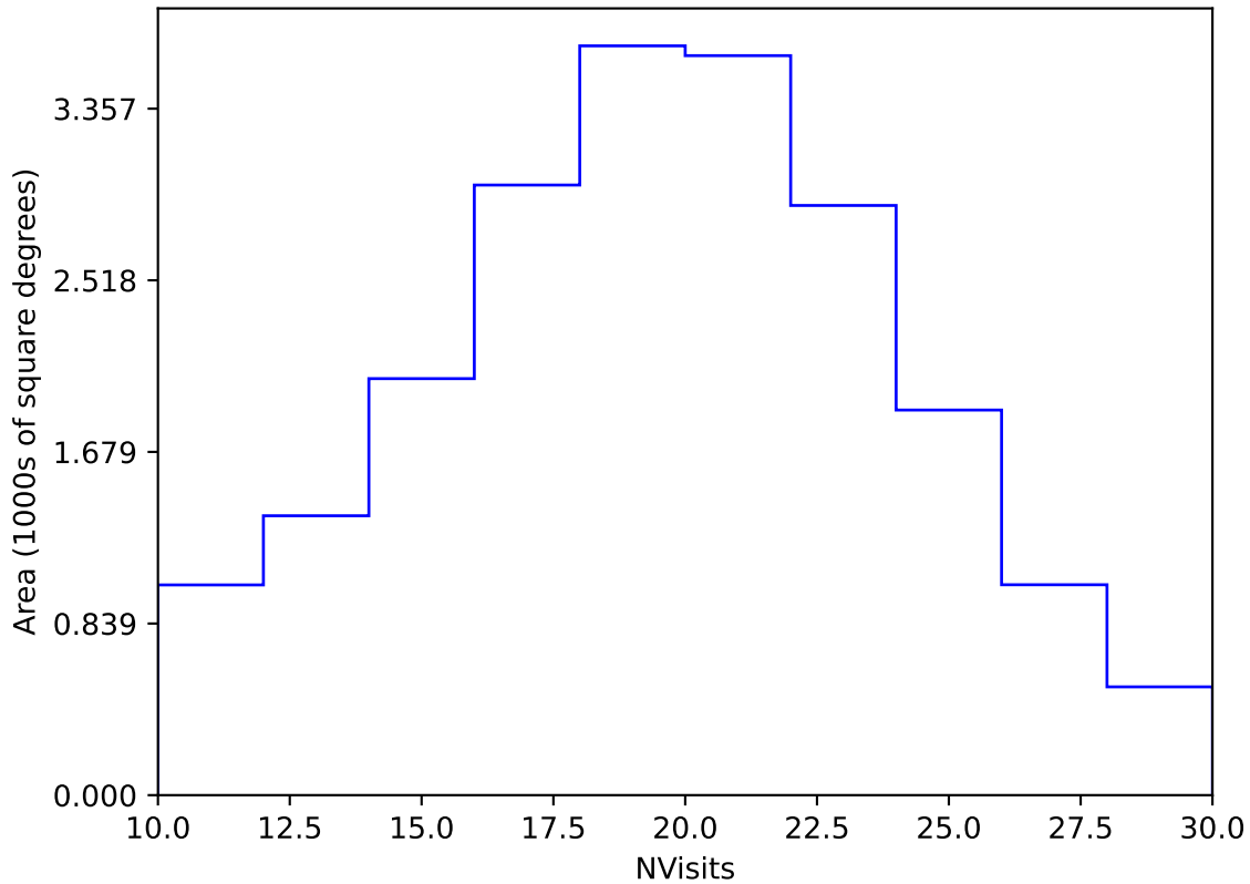
ddf_loaded_fl15_v3.4_10yrs Yr 1 y band: NVisits
