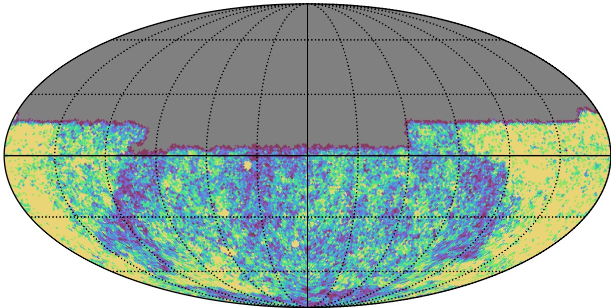
ddf_loaded_fl15_v3.4_10yrs Yr 1 u band: NVisits
