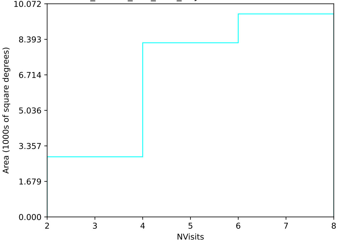
ddf_loaded_fl15_v3.4_10yrs Yr 1 u band: NVisits
