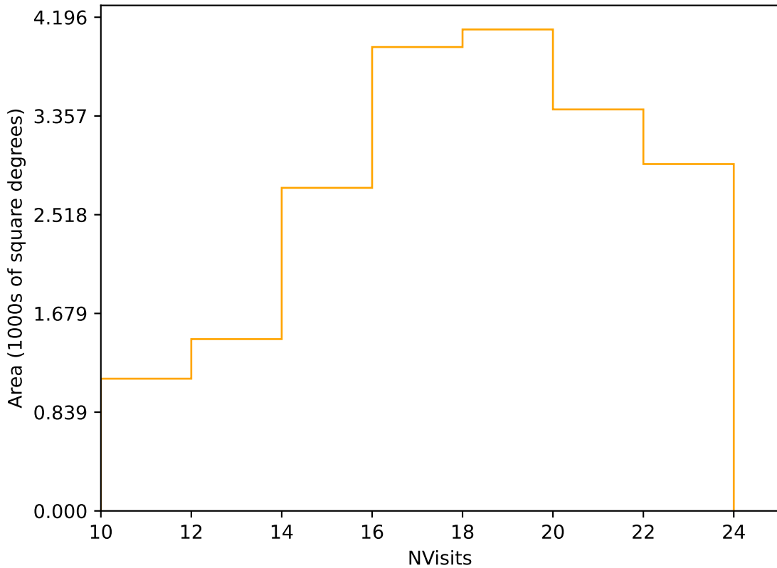
ddf_loaded_fl15_v3.4_10yrs Yr 1 r band: NVisits
