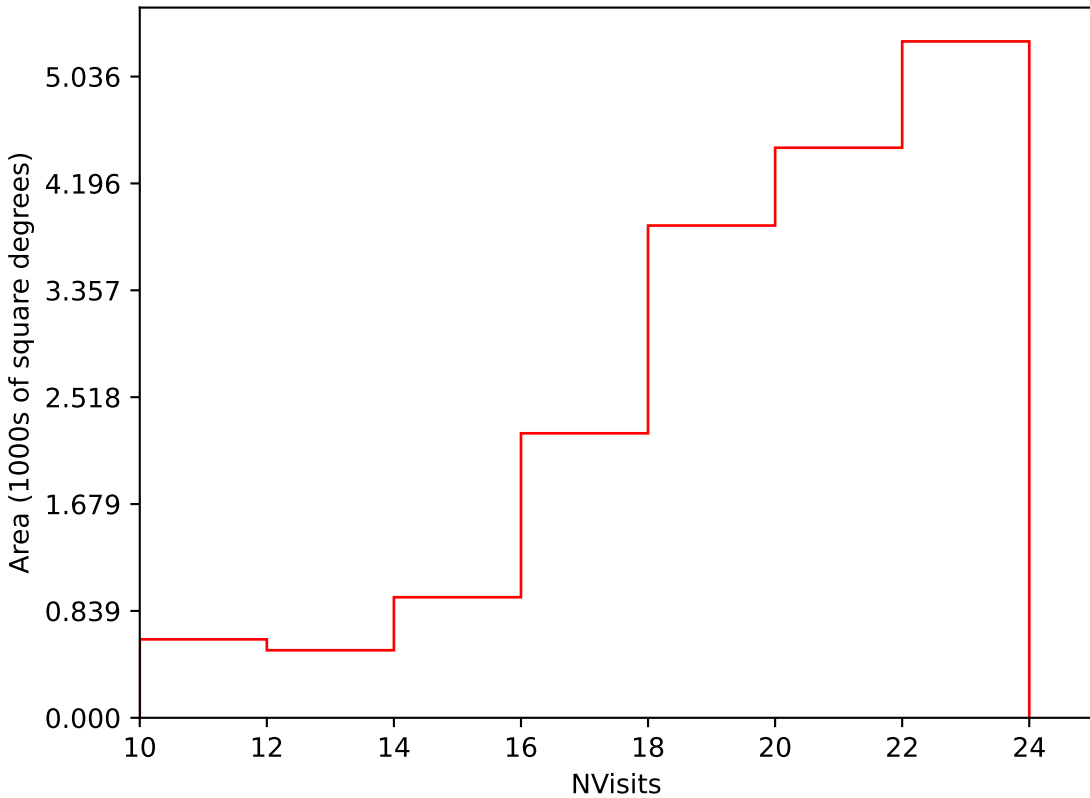
ddf_loaded_fl15_v3.4_10yrs Yr 1 i band: NVisits
