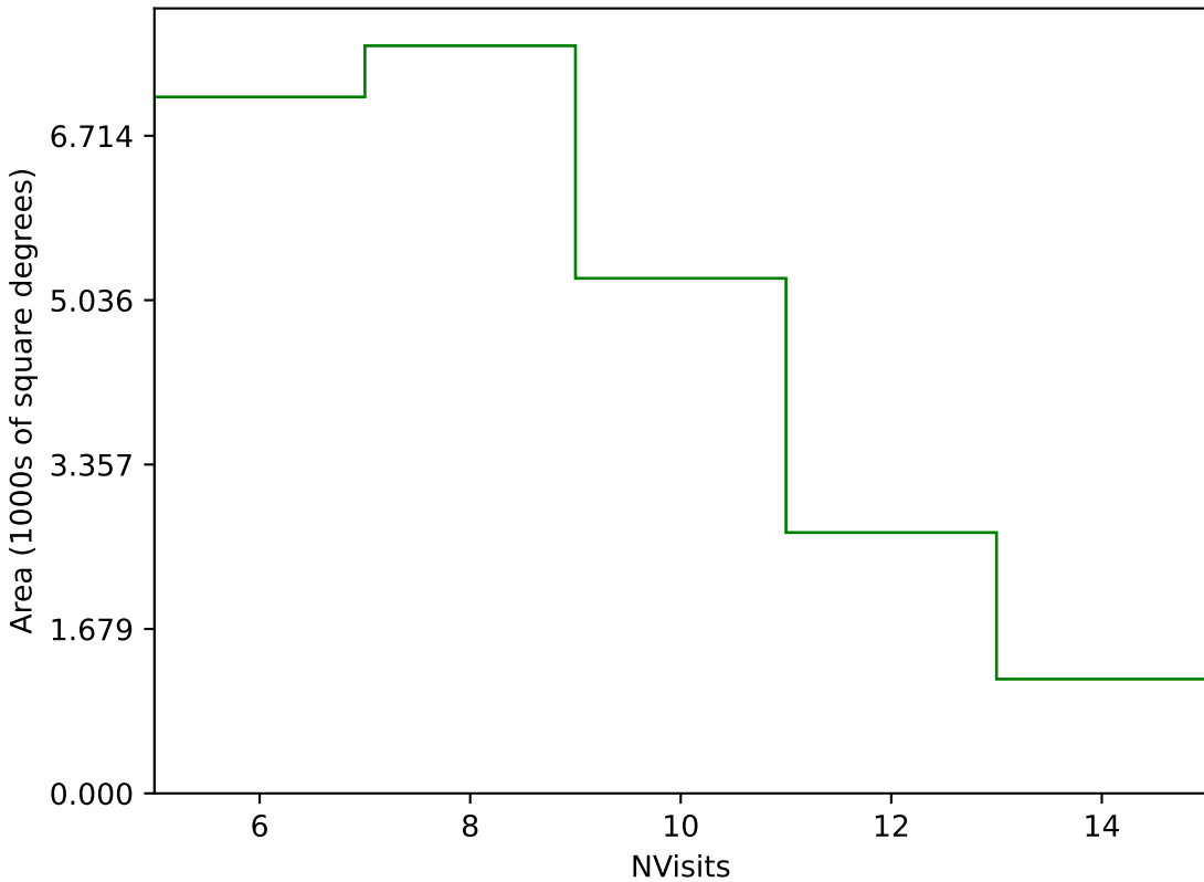
ddf_loaded_fl15_v3.4_10yrs Yr 1 g band: NVisits
