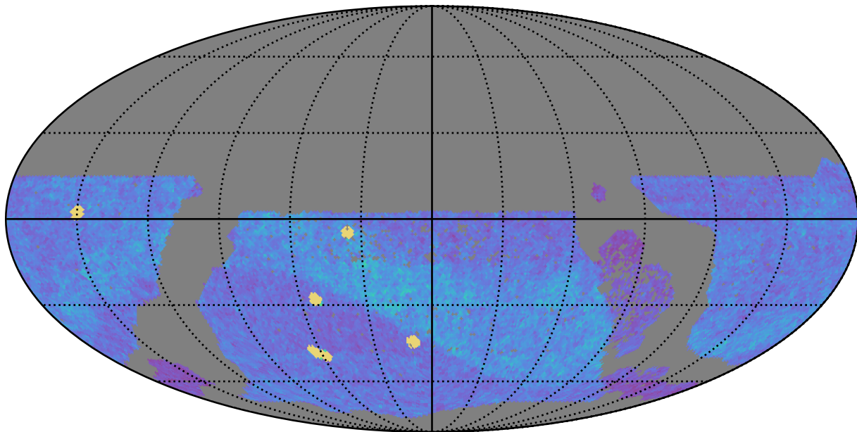
ddf_loaded_fl15_v3.4_10yrs WFD z band: NVisits
