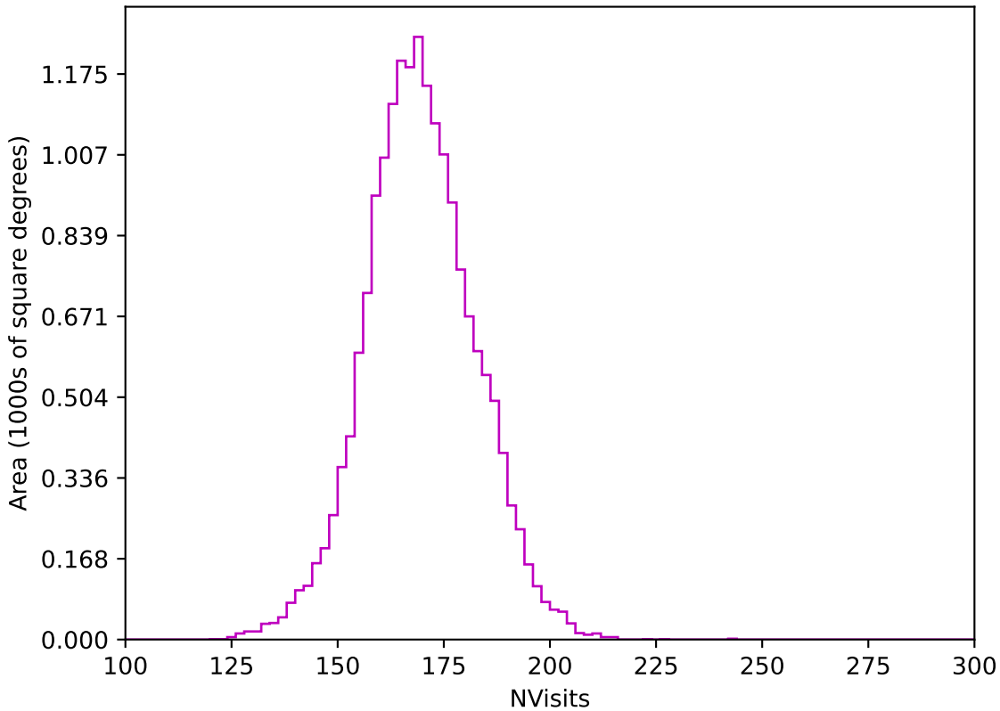
ddf_loaded_fl15_v3.4_10yrs WFD z band: NVisits
