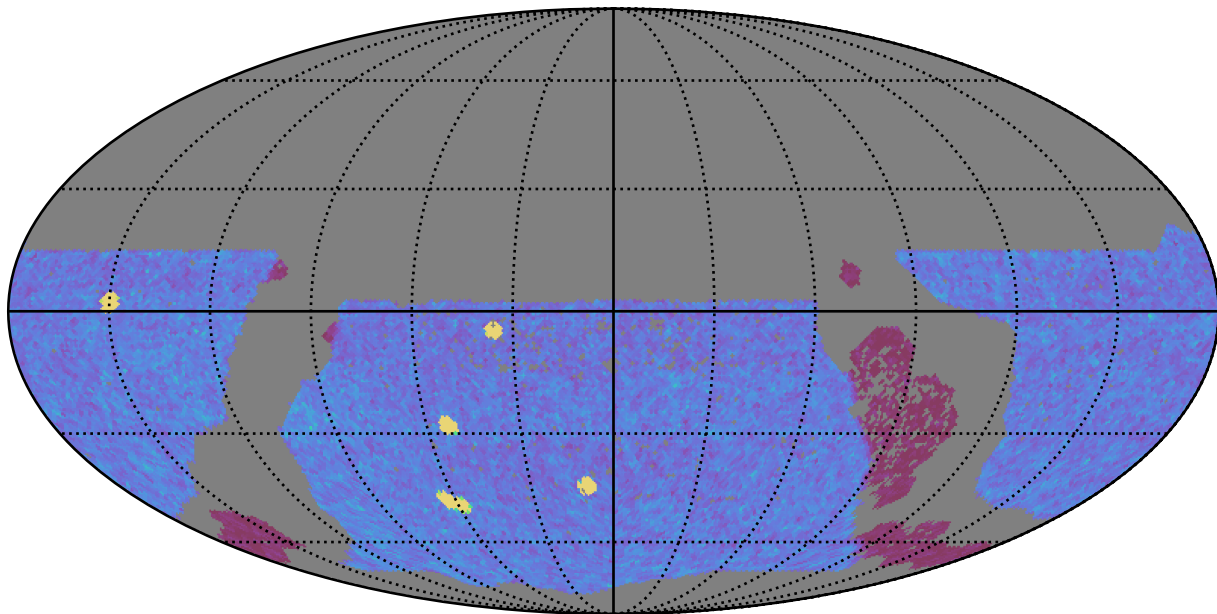
ddf_loaded_fl15_v3.4_10yrs WFD y band: NVisits
