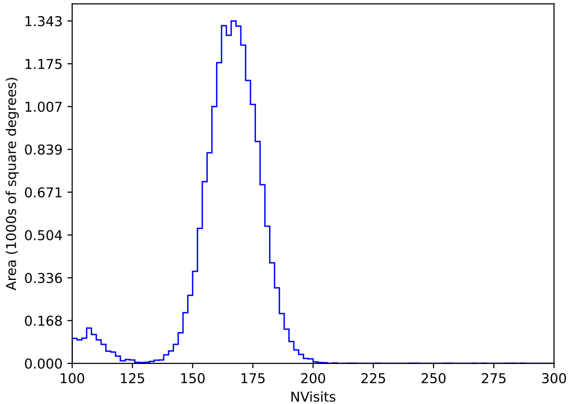
ddf_loaded_fl15_v3.4_10yrs WFD y band: NVisits
