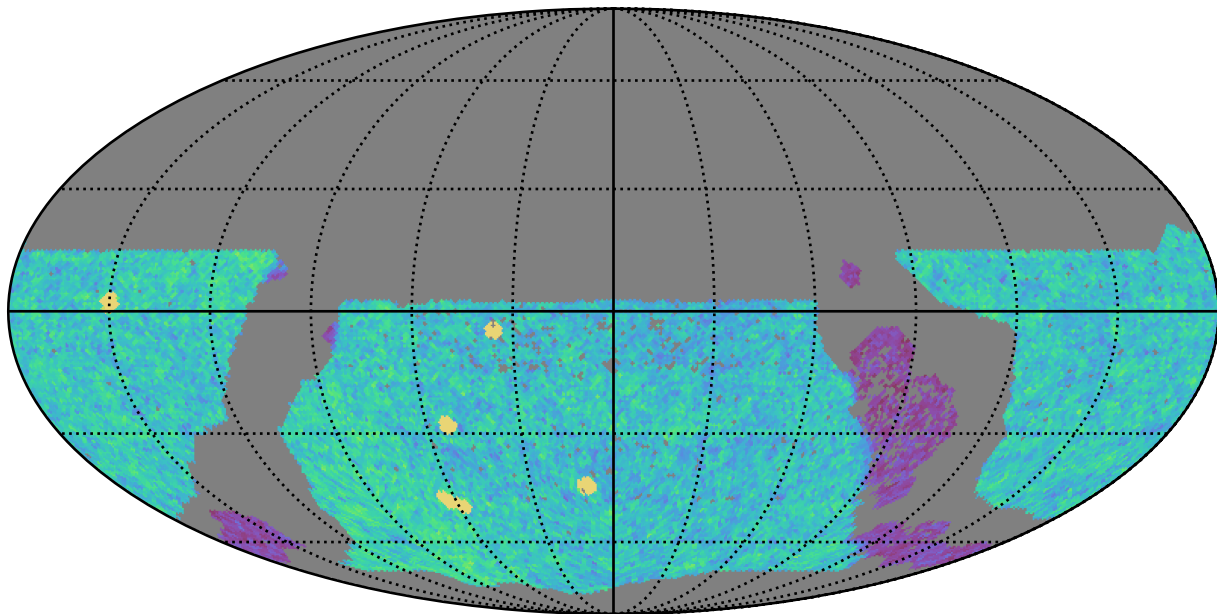
ddf_loaded_fl15_v3.4_10yrs WFD u band: NVisits
