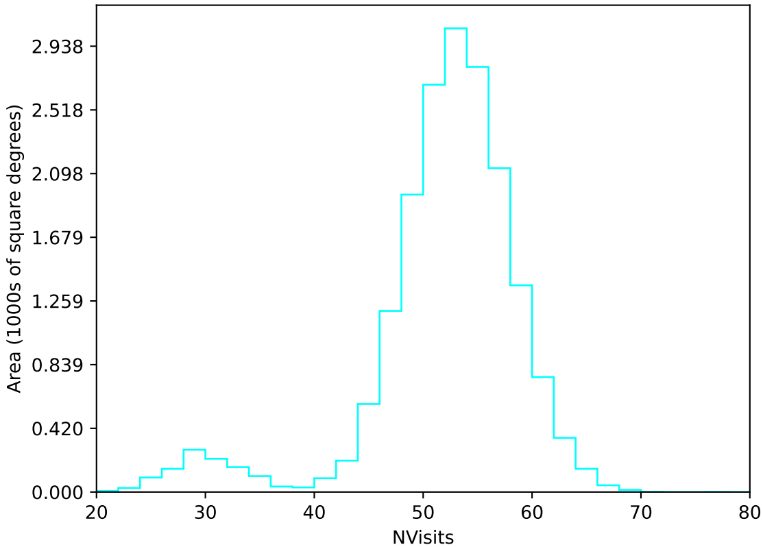
ddf_loaded_fl15_v3.4_10yrs WFD u band: NVisits
