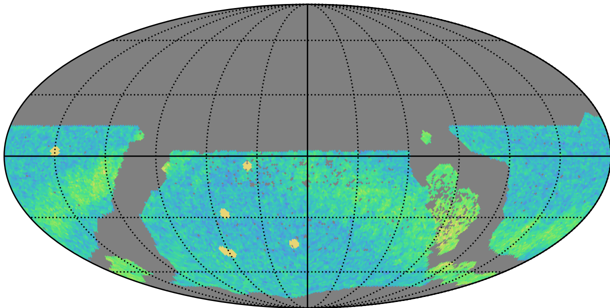
ddf_loaded_fl15_v3.4_10yrs WFD r band: NVisits
