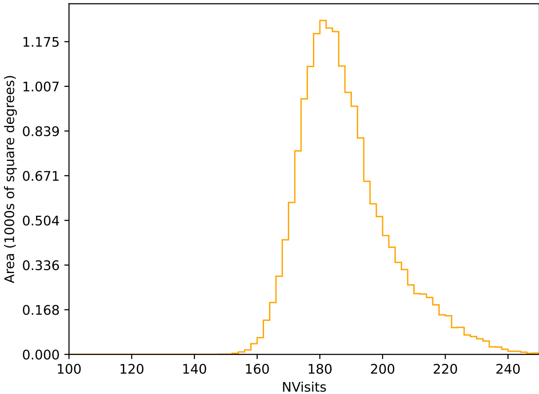
ddf_loaded_fl15_v3.4_10yrs WFD r band: NVisits
