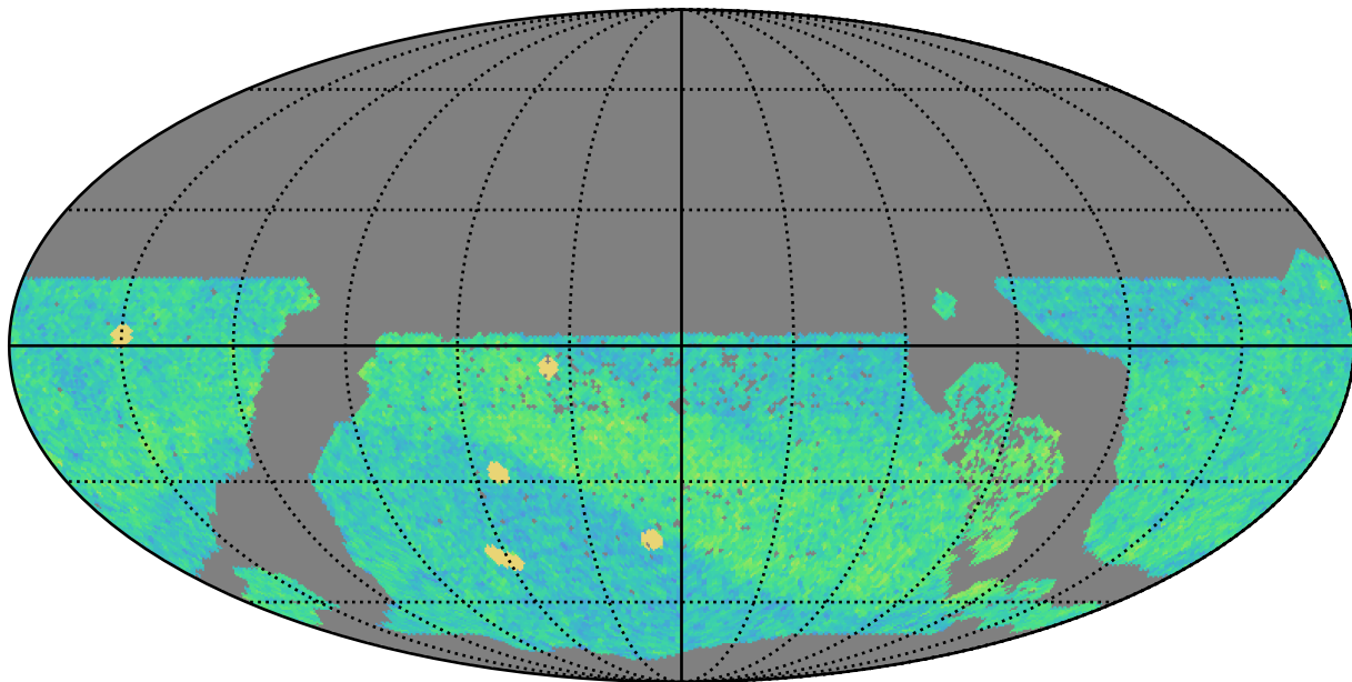
ddf_loaded_fl15_v3.4_10yrs WFD i band: NVisits
