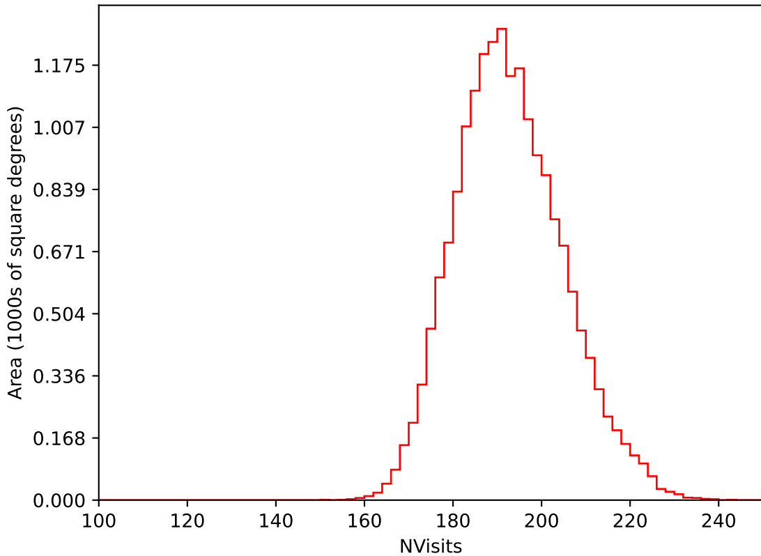
ddf_loaded_fl15_v3.4_10yrs WFD i band: NVisits
