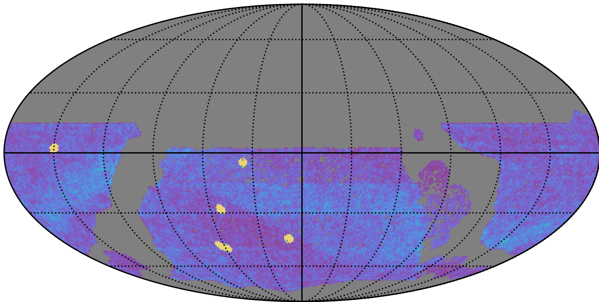
ddf_loaded_fl15_v3.4_10yrs WFD all bands: NVisits
