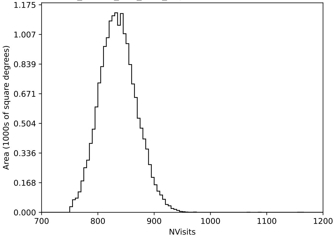
ddf_loaded_fl15_v3.4_10yrs WFD all bands: NVisits
