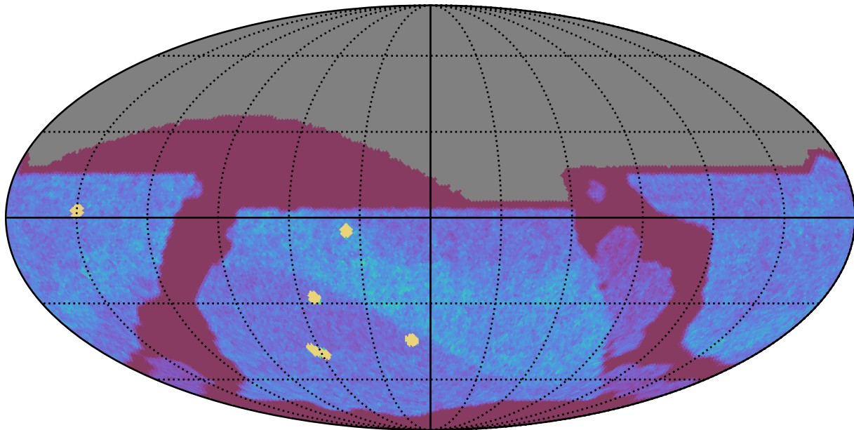
ddf_loaded_fl15_v3.4_10yrs All sky z band: NVisits
