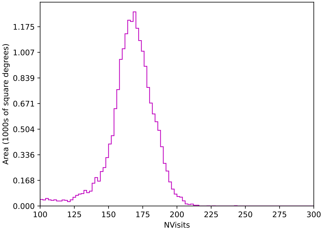
ddf_loaded_fl15_v3.4_10yrs All sky z band: NVisits
