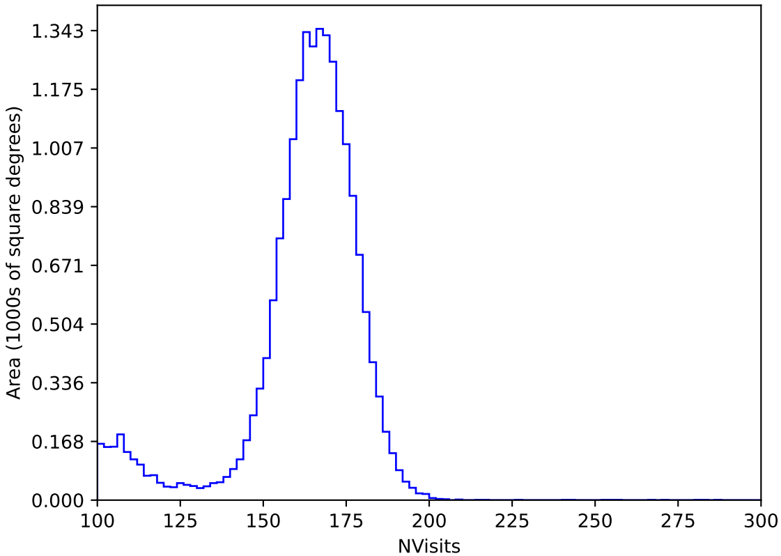
ddf_loaded_fl15_v3.4_10yrs All sky y band: NVisits
