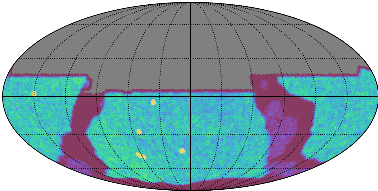
ddf_loaded_fl15_v3.4_10yrs All sky u band: NVisits
