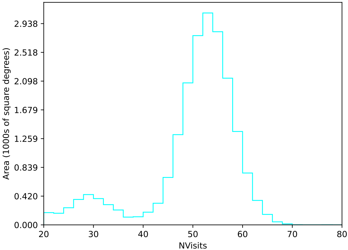
ddf_loaded_fl15_v3.4_10yrs All sky u band: NVisits
