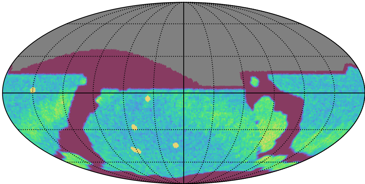
ddf_loaded_fl15_v3.4_10yrs All sky r band: NVisits
