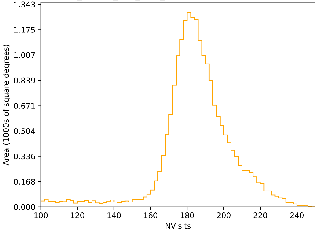
ddf_loaded_fl15_v3.4_10yrs All sky r band: NVisits
