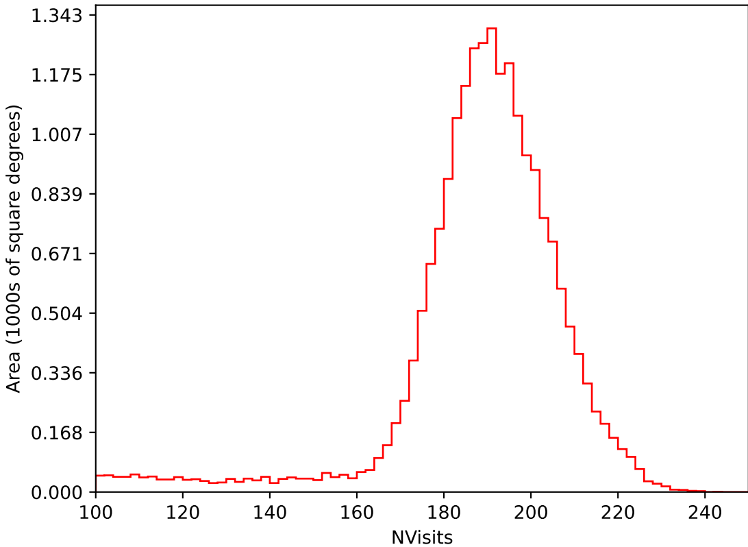
ddf_loaded_fl15_v3.4_10yrs All sky i band: NVisits
