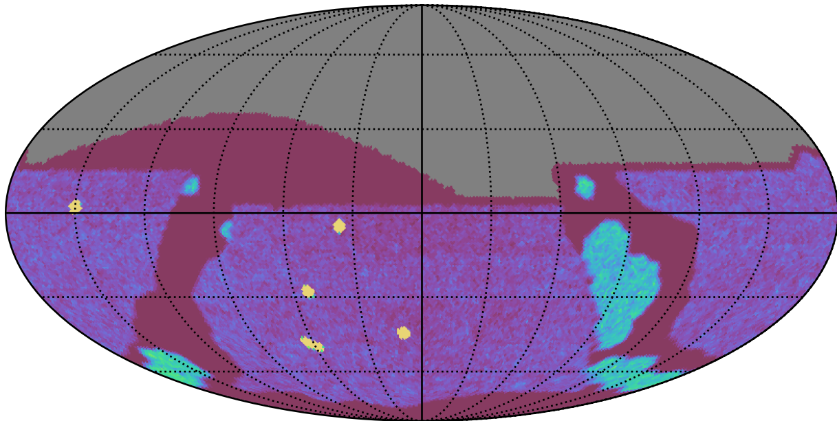
ddf_loaded_fl15_v3.4_10yrs All sky g band: NVisits
