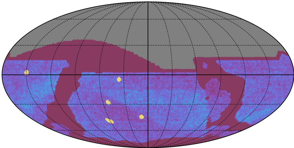
ddf_loaded_fl15_v3.4_10yrs All sky all bands: NVisits
