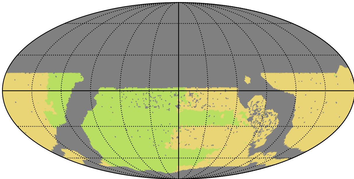
ddf_loaded_fl15_v3.4_10yrs WFD all bands: NSeasons
