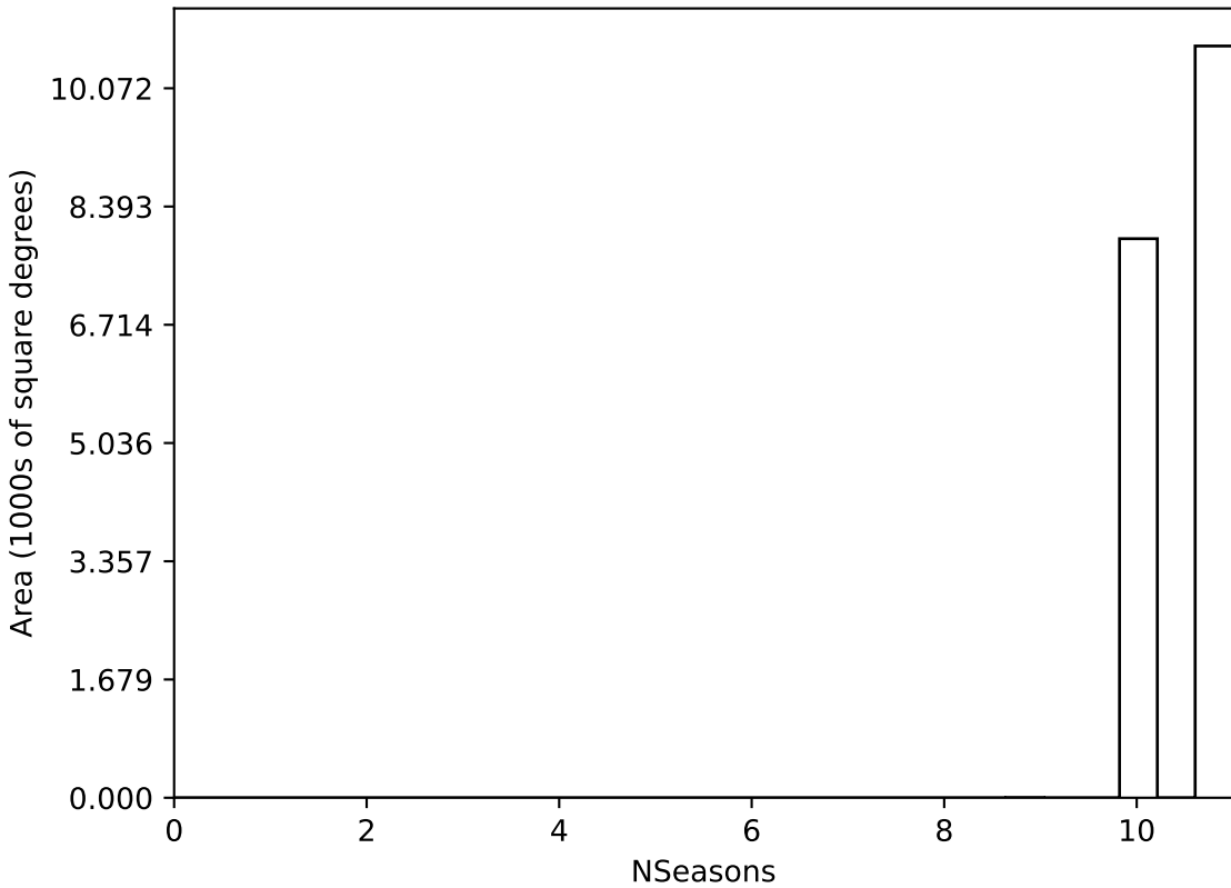
ddf_loaded_fl15_v3.4_10yrs WFD all bands: NSeasons
