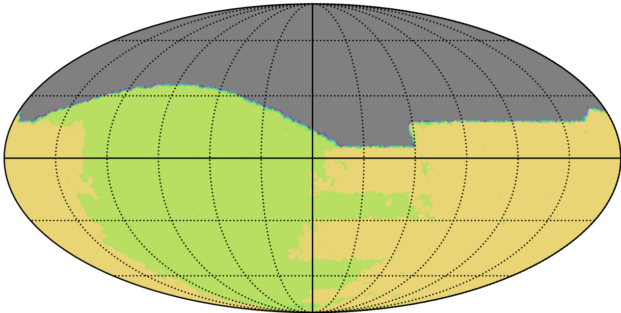
ddf_loaded_fl15_v3.4_10yrs All sky all bands: NSeasons
