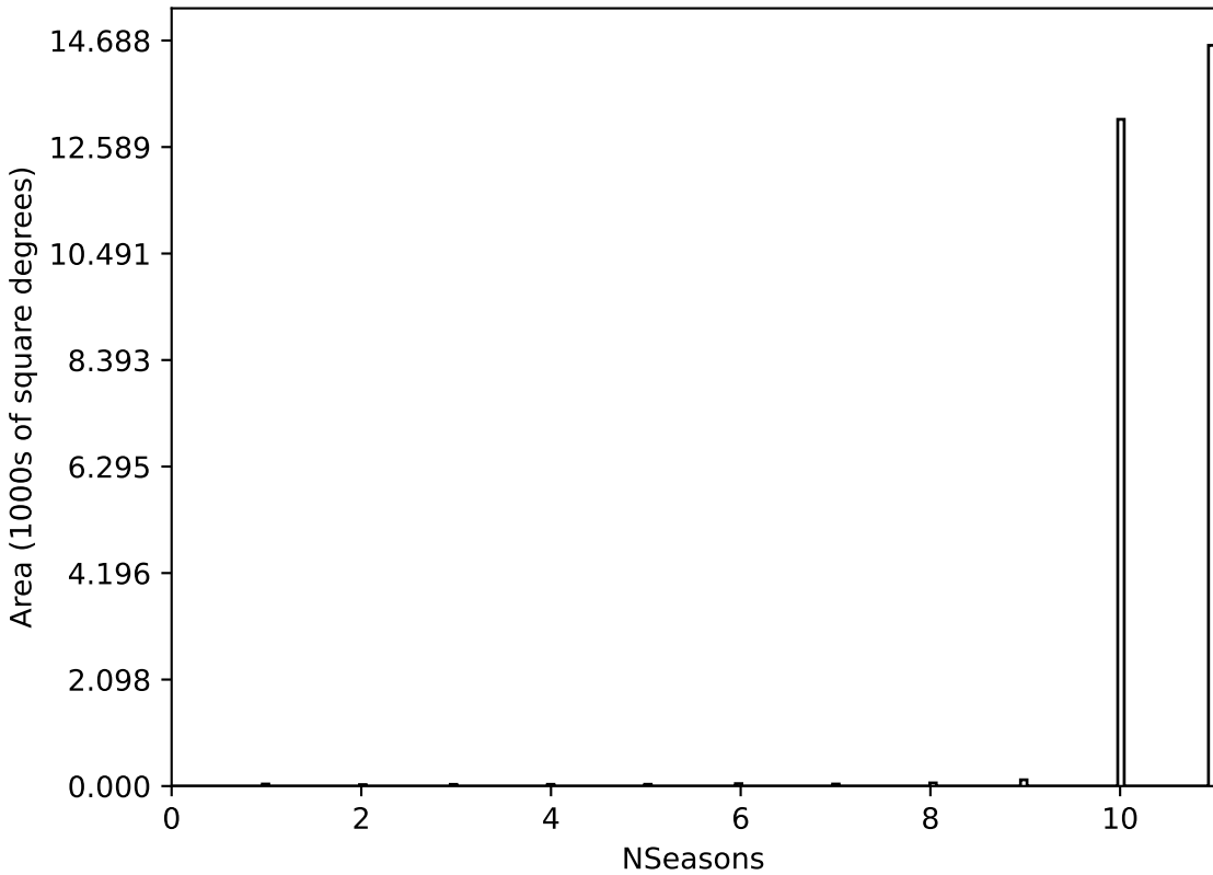
ddf_loaded_fl15_v3.4_10yrs All sky all bands: NSeasons
