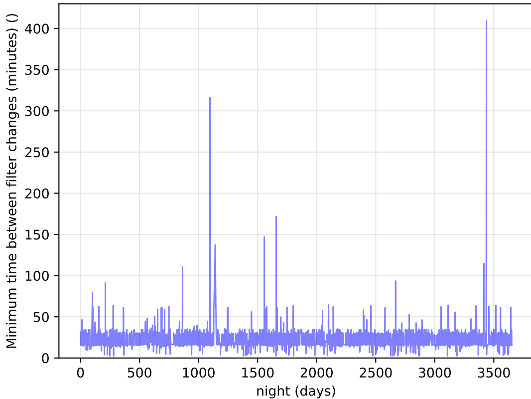
ddf_loaded_fl15_v3.4_10yrs Per Night: Minimum time between filter changes (minutes)
