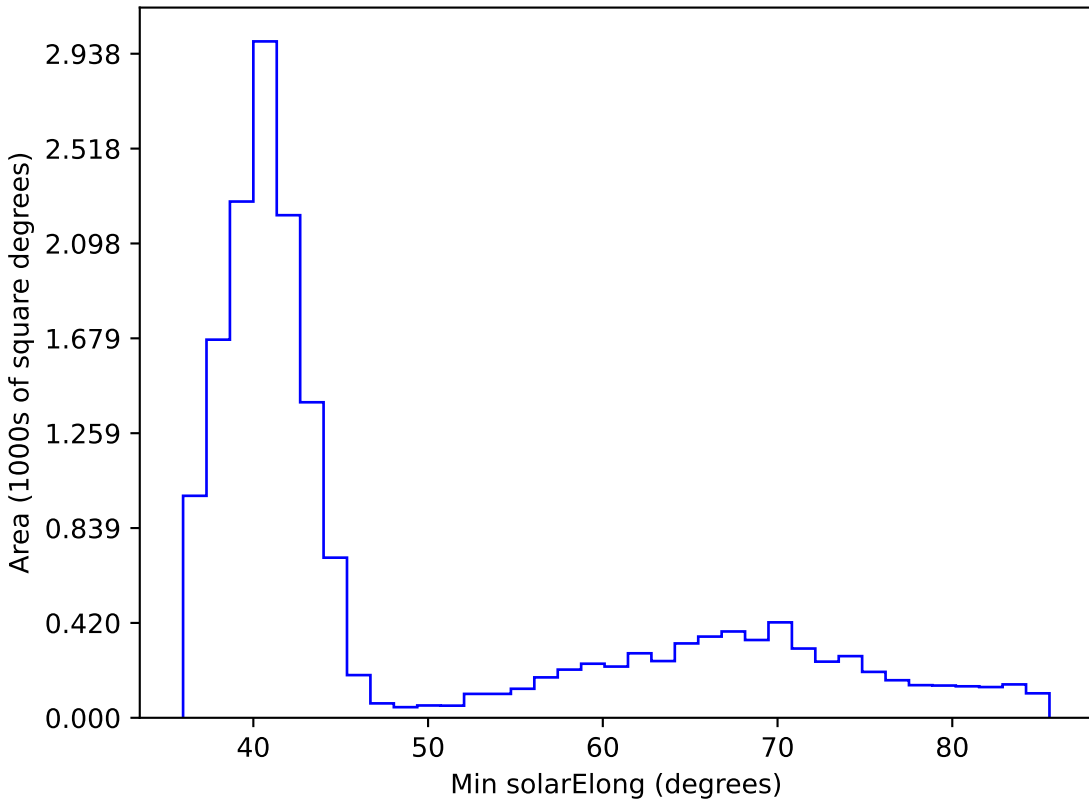
ddf_loaded_fl15_v3.4_10yrs WFD z band: Min solarElong
