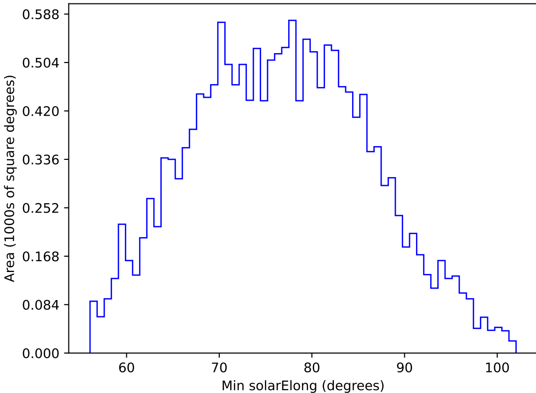
ddf_loaded_fl15_v3.4_10yrs WFD u band: Min solarElong
