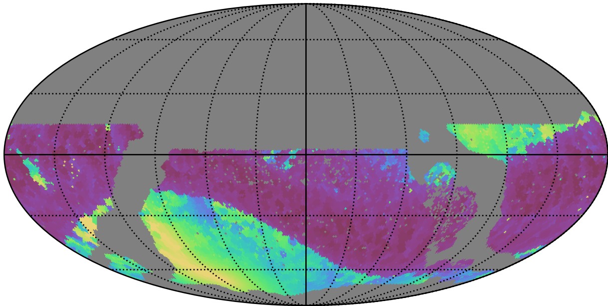
ddf_loaded_fl15_v3.4_10yrs WFD i band: Min solarElong
