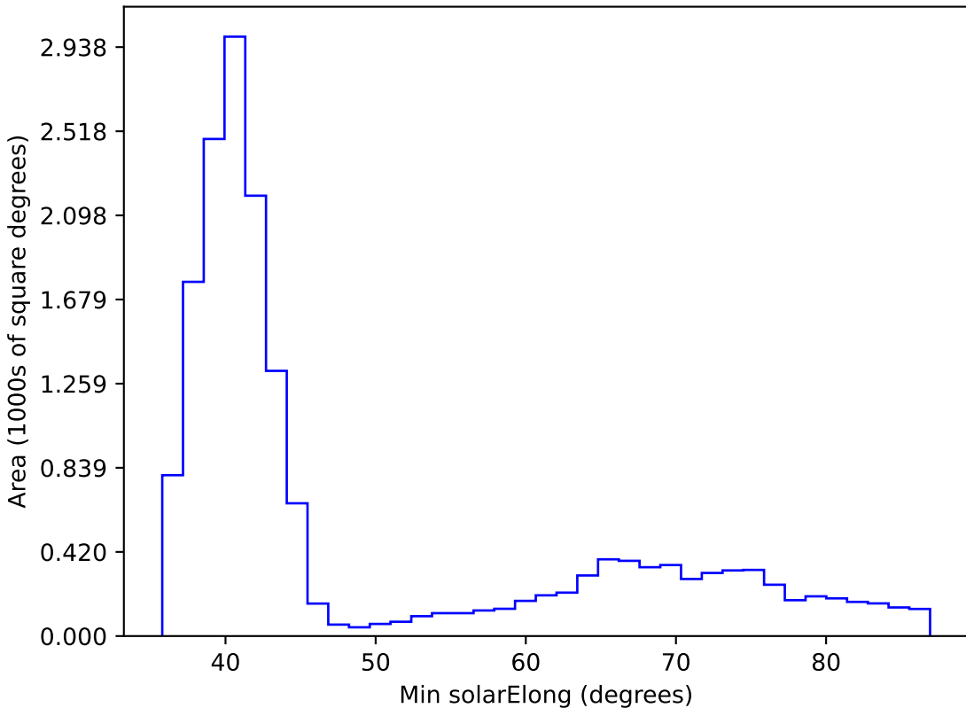
ddf_loaded_fl15_v3.4_10yrs WFD i band: Min solarElong
