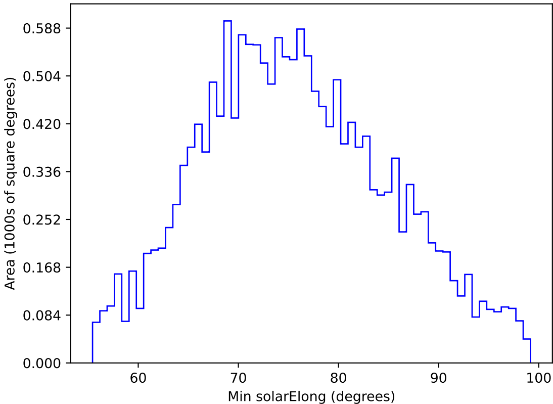
ddf_loaded_fl15_v3.4_10yrs WFD g band: Min solarElong
