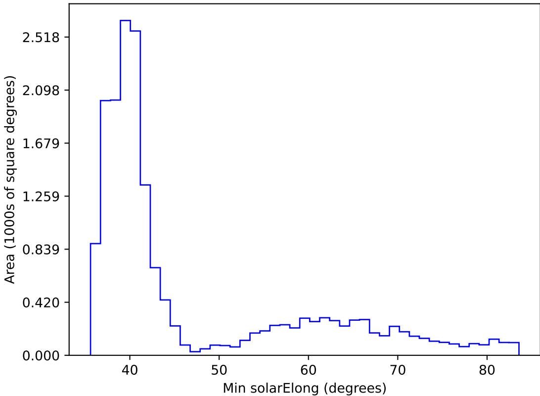
ddf_loaded_fl15_v3.4_10yrs WFD all bands: Min solarElong
