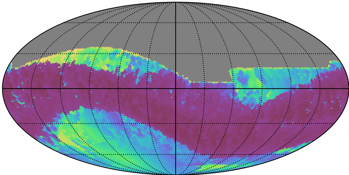
ddf_loaded_fl15_v3.4_10yrs All sky z band: Min solarElong
