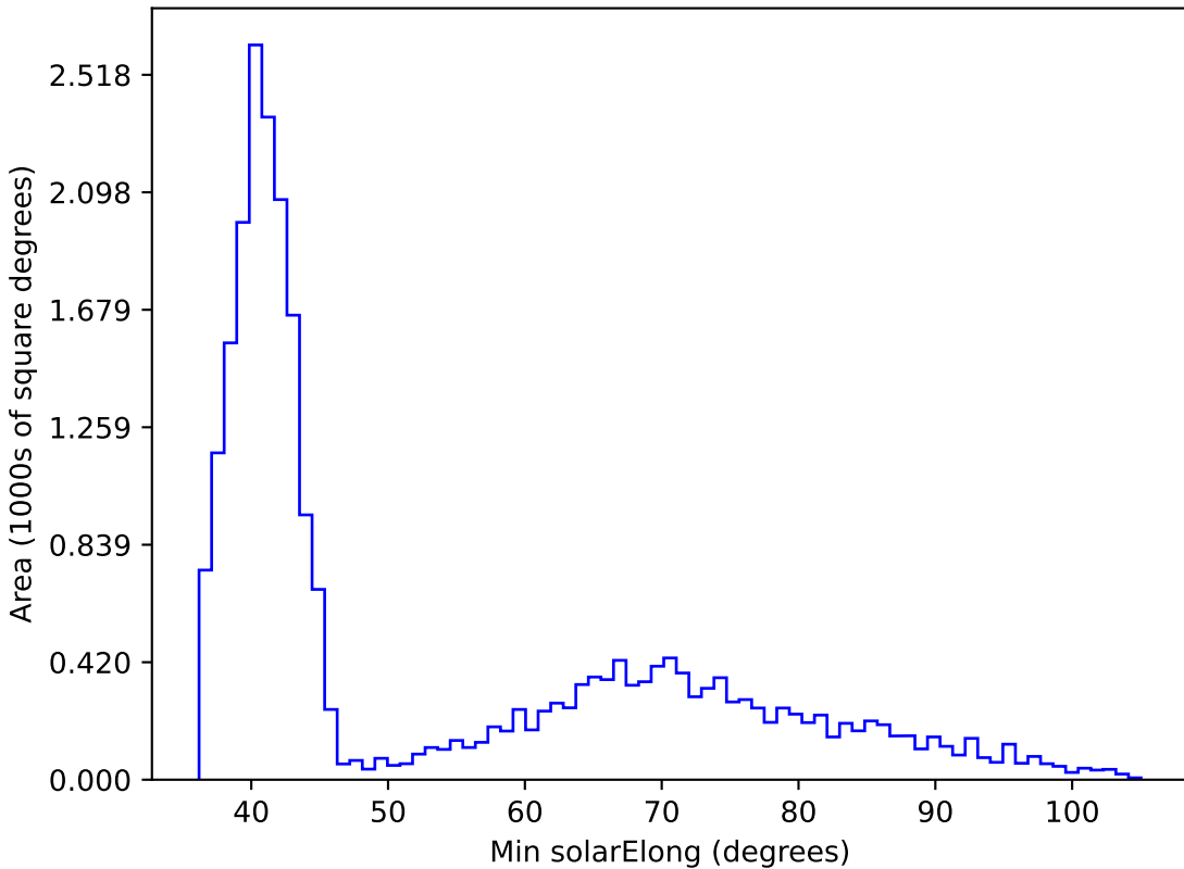
ddf_loaded_fl15_v3.4_10yrs All sky z band: Min solarElong
