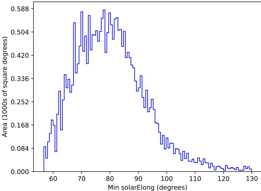
ddf_loaded_fl15_v3.4_10yrs All sky u band: Min solarElong
