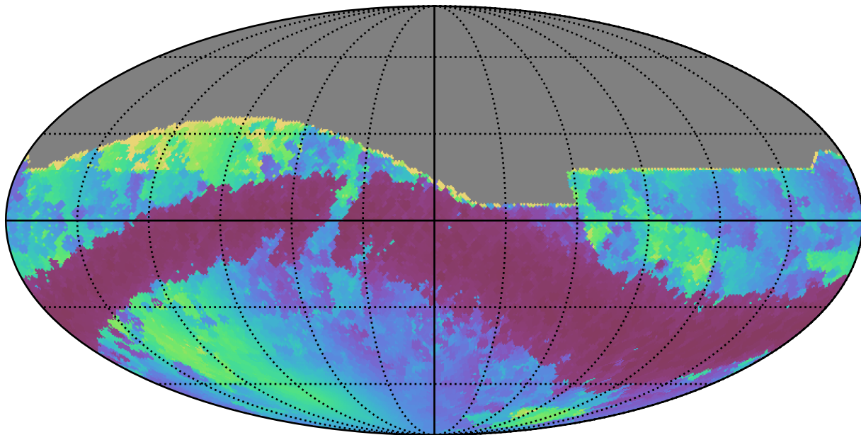
ddf_loaded_fl15_v3.4_10yrs All sky r band: Min solarElong
