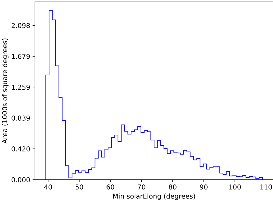
ddf_loaded_fl15_v3.4_10yrs All sky r band: Min solarElong
