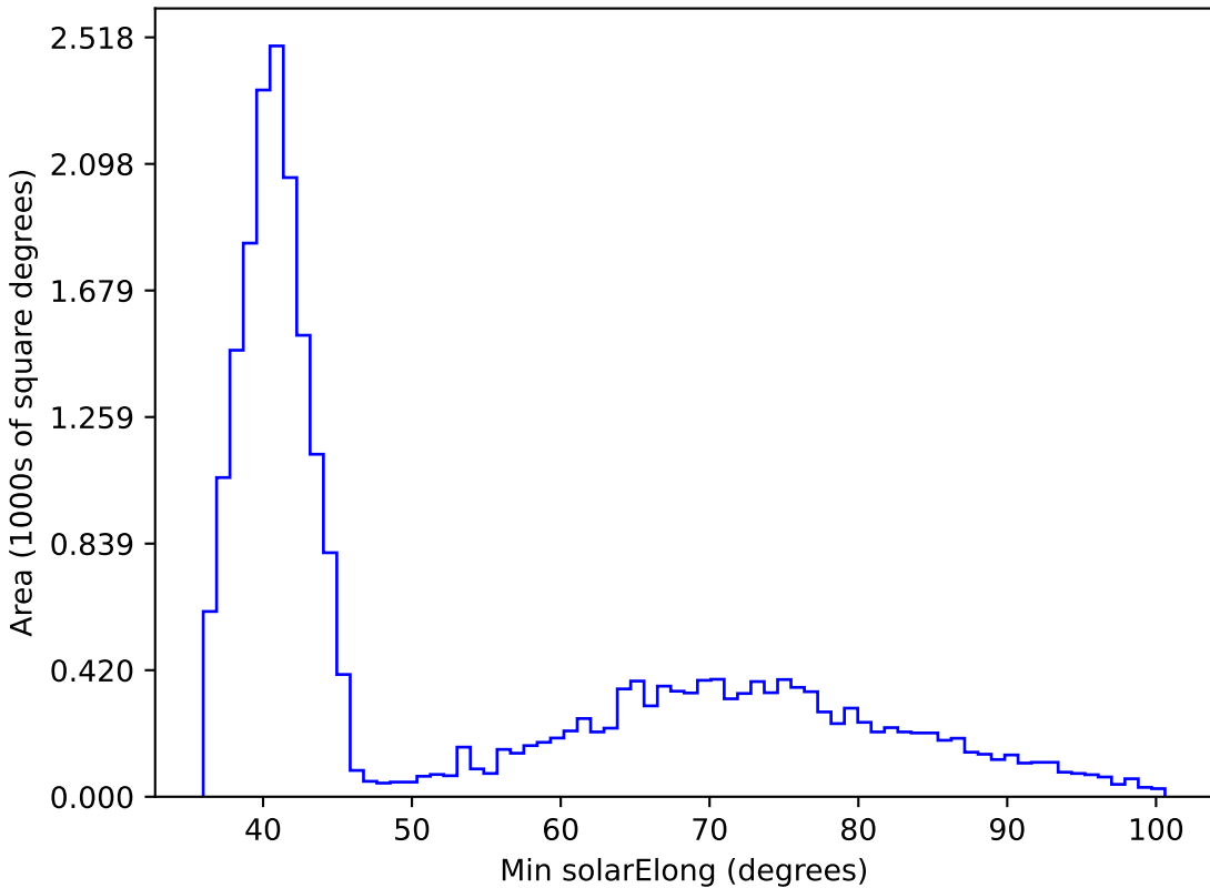
ddf_loaded_fl15_v3.4_10yrs All sky i band: Min solarElong
