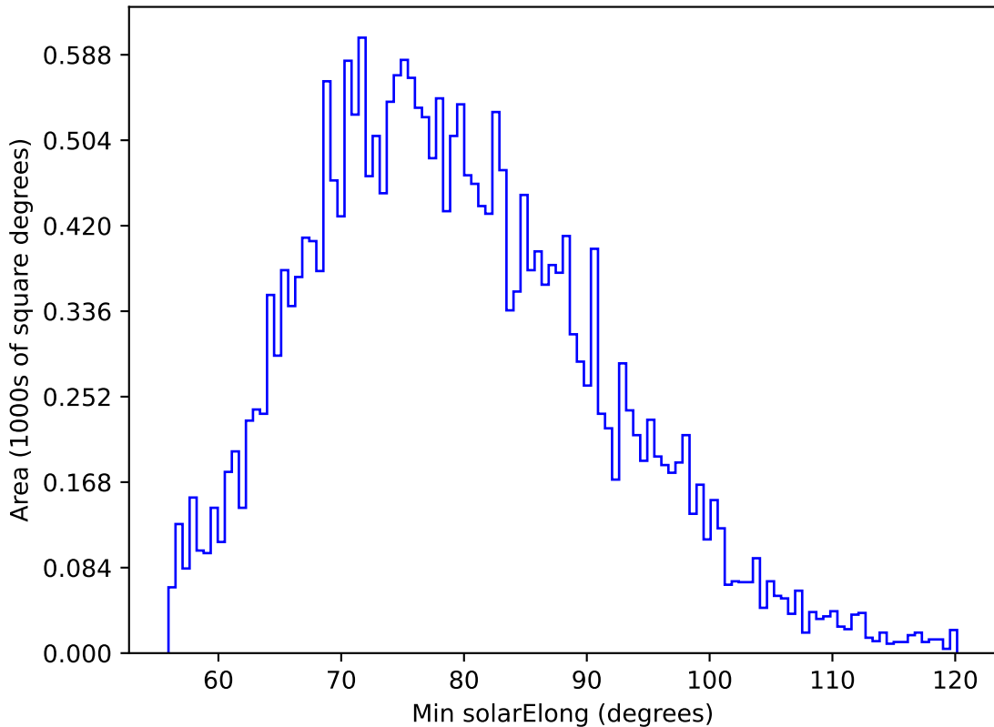
ddf_loaded_fl15_v3.4_10yrs All sky g band: Min solarElong
