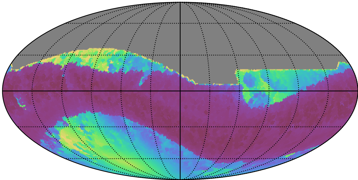
ddf_loaded_fl15_v3.4_10yrs All sky all bands: Min solarElong
